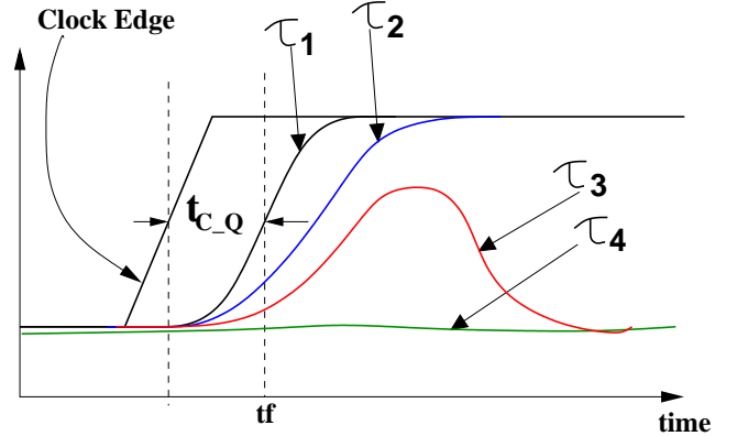
(a) Output for \tau_1 > \tau_2 > \tau_3 > \tau_4 .
