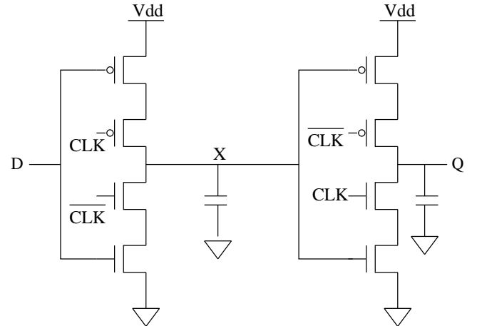
Fig. 6. C^2 MOS Positive-edge triggered master-slave register.
