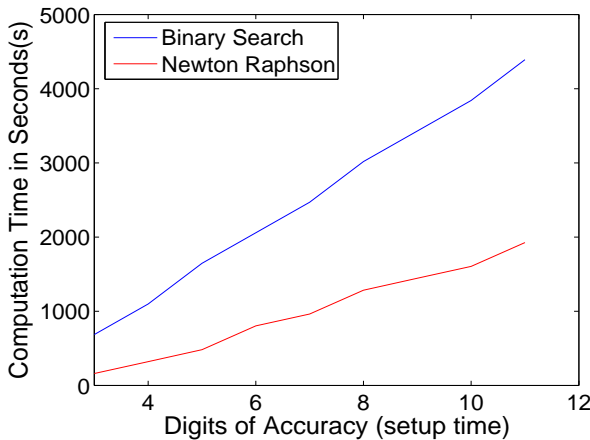
(b) Computation Time vs Digits of Accuracy.
