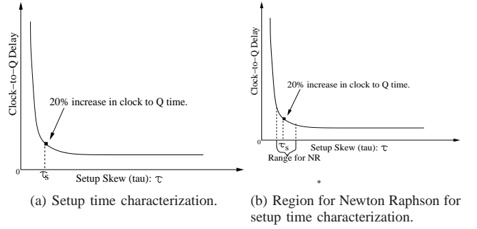
Fig. 3. Setup skew vs clock-to-output delay
