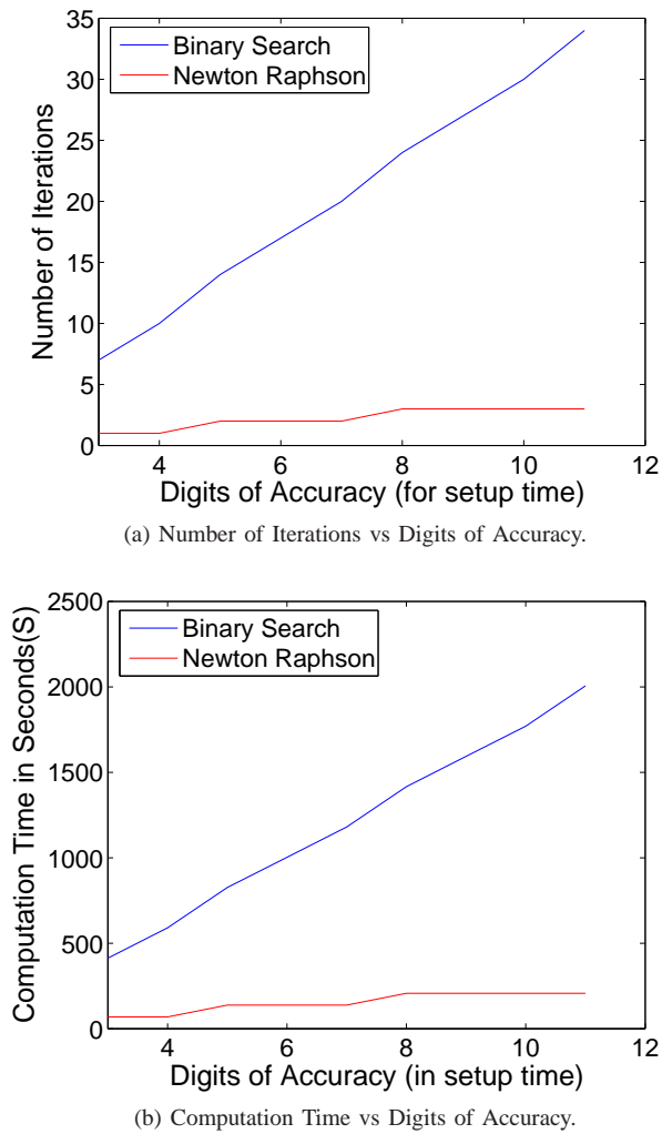
Fig. 7. Digits of Accuracy: Newton Raphson vs Binary Search Method.
