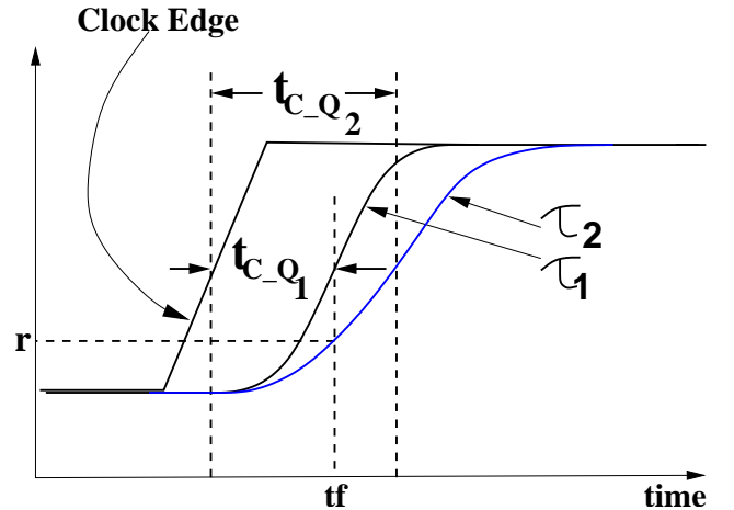
(b) Clock to Q delay.
